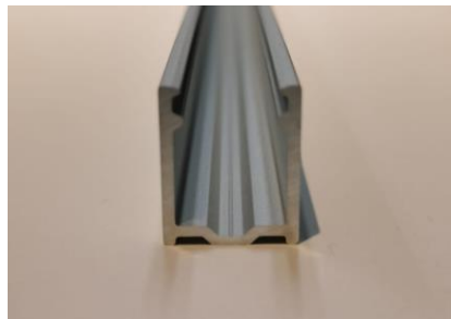
Aluminium Profile: 1000x14.4x21.4mm
